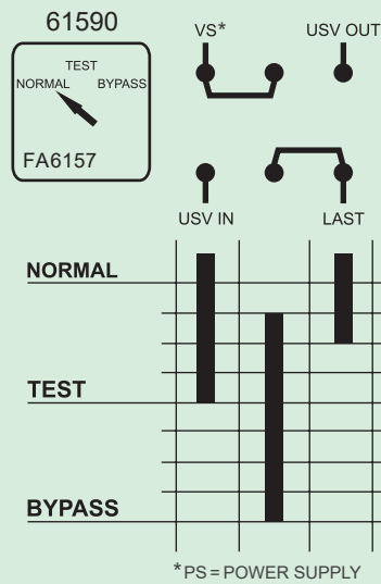
Bypass switch with 3 switch positions "NORMAL – TEST – BYPASS" (1-pole)
